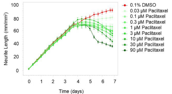
Figure 4: iCell Sensory Neurons were cultured for four days followed by a 3-day treatment with varying doses of Paclitaxel, a chemotherapeutic with known CIPN-inducing side effects. iCell Sensory Neurons display a dose-response neurite degeneration to Paclitaxel.
