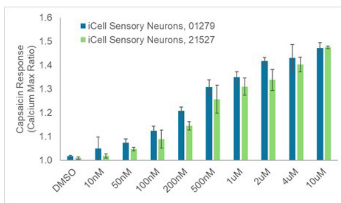
Figure 6: iCell Sensory Neurons from both 01279 (male) and 21527 (female) cell lines were cultured for 21 days and a dose-response to capsaicin, using calcium imaging, was performed. Data show similar response kinetics between 01279 and 21527 donors.
